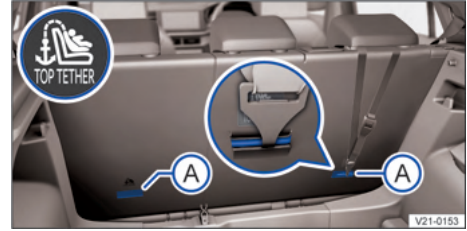
Mounting eyelets on the rear seats
